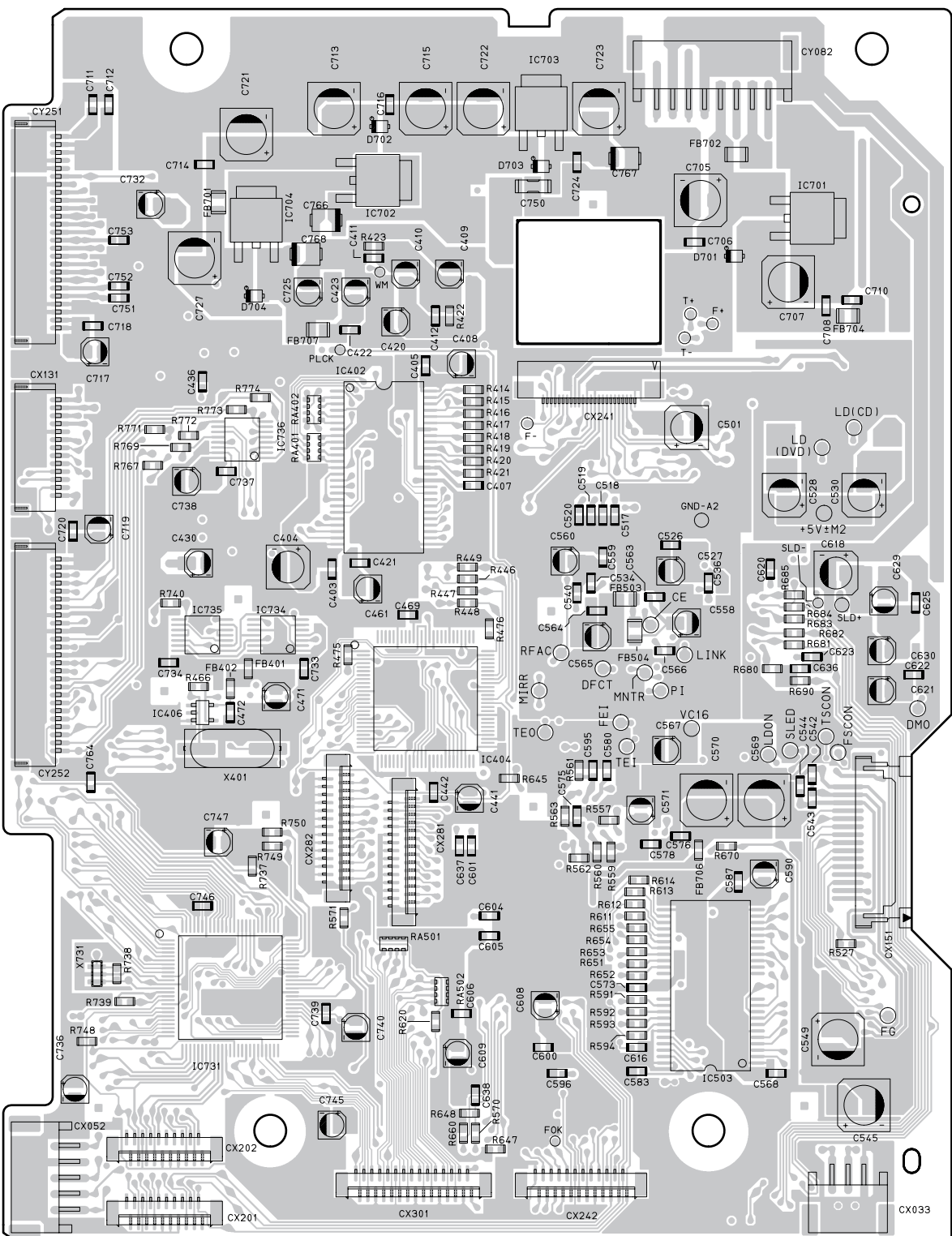
FOIL SIDE
