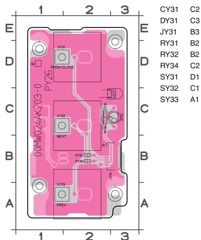
PY26 PCB
