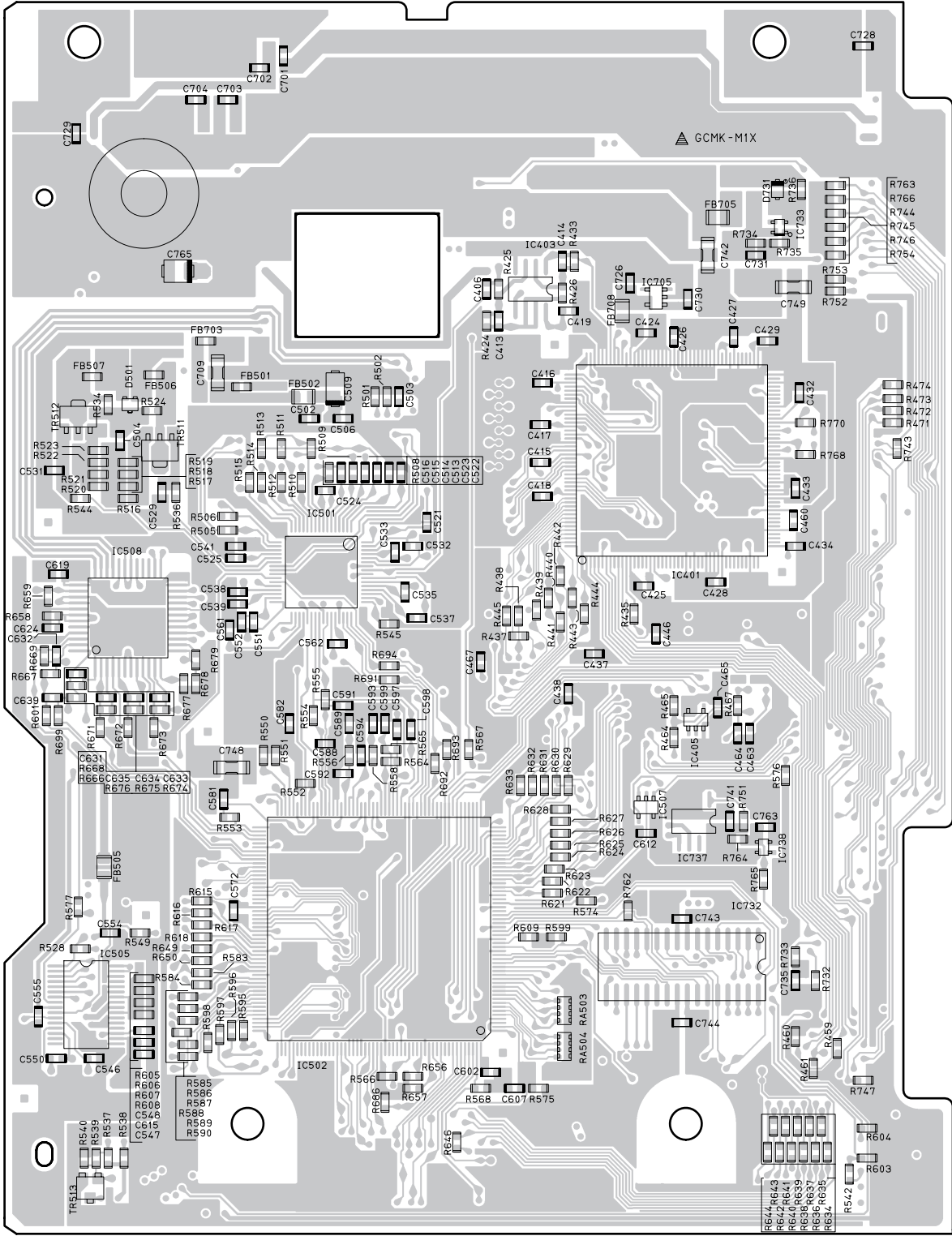
COMPONENT SIDE
